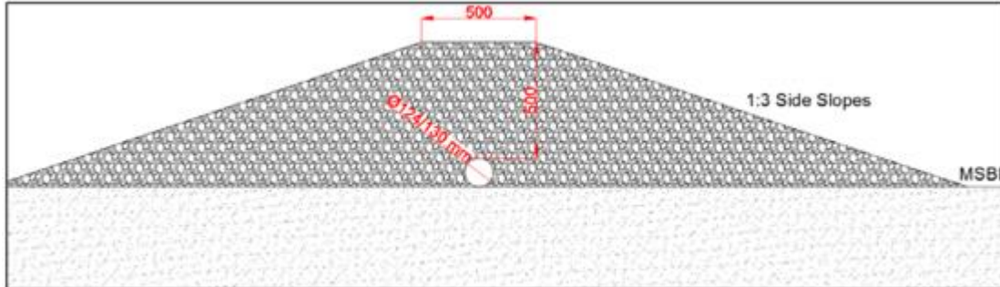
Fig. 6 Rock Berm Profile – Surface Laid Section (worse case)
